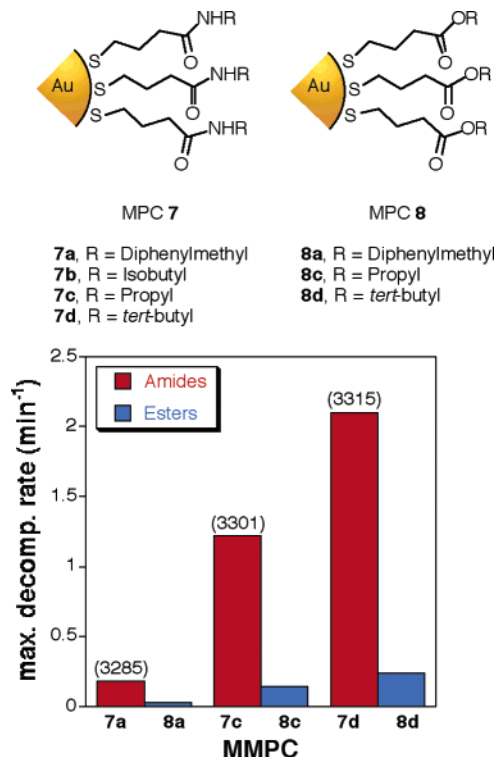
FIGURE 5. Maximal NaCN decomposition rates of amide- and corresponding ester-functionalized MPCs. For comparison, N–H stretching frequencies ( \text{cm}^{-1} ) of the corresponding amide-functionalized MPCs are given in parentheses.
